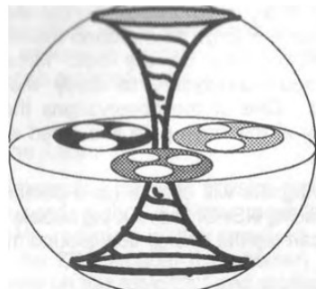
Figure 1.2.2-1. Keely "Atom" (i.e., Proton) Showing Torroidal Structure
